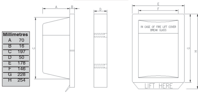
STOPPER II Dimensions
