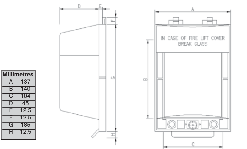
STOPPER II Dimensions
